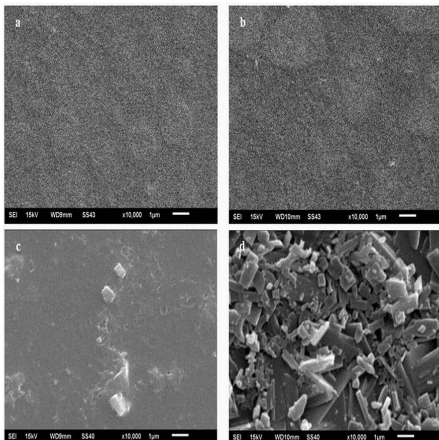
Figure 3-3. SEM of surface of the edible gallic acid-chitosan and chitosan-only films (a. represents the edible film casted from chitosan without gallic acid; b. represents edible film casted from chitosan with 0.5 g/100 g gallic acid (w/v); c. represents edible film casted from chitosan with 1.0 g/100 g gallic acid (w/v); d. represents edible film casted from chitosan with 1.5 g/100 g gallic acid (w/v)).
