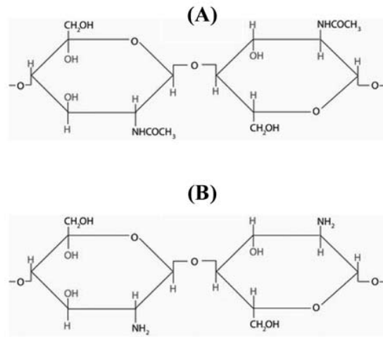
Figure 1-1. Structure of (A) chitin and (B) chitosan ((Muzzarelli 1996)
