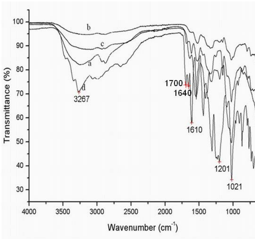
Figure 3- 2. FT-IR spectra of the edible gallic acid-chitosan and chitosan-only films (a. represents the edible film casted from chitosan without gallic acid; b. represents edible film casted from chitosan with 0.5 g/100 g gallic acid (w/v); c. represents edible film casted from chitosan with 1.0 g/100 g gallic acid (w/v); d. represents edible film casted from chitosan with 1.5 g/100 g gallic acid (w/v)).
